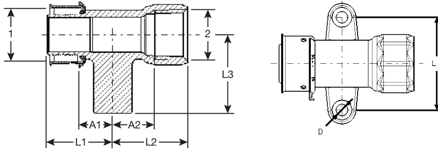
Viega PEX Press Adapter Zero Lead Bronze for Fire Sprinkler System P x FPT - Model 2812.2ZL
