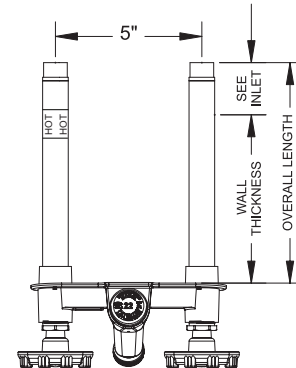
Model 22 Rough-In Dimensions
